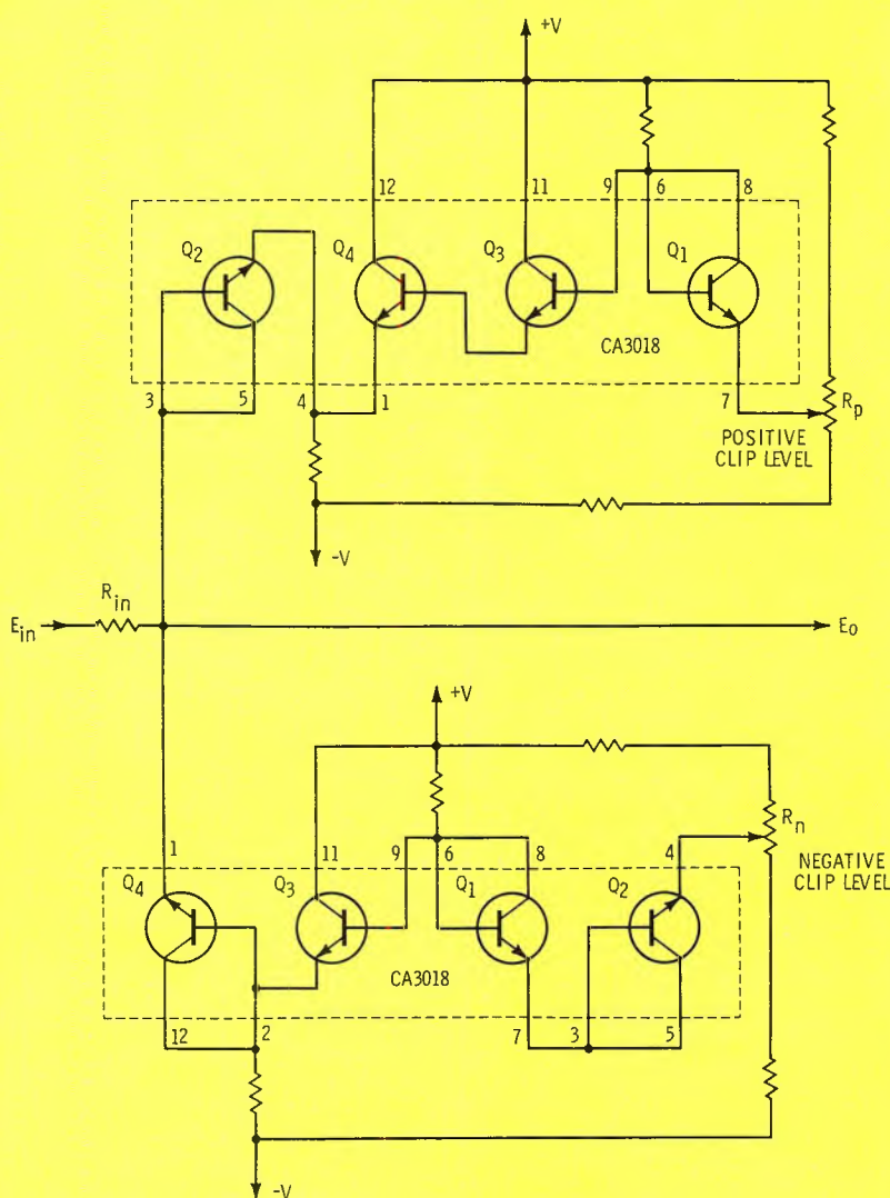
Fig. 3d Bi-directional clipper.
