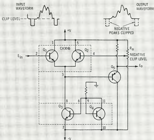
Fig. 3b Negative (black) limiter.
