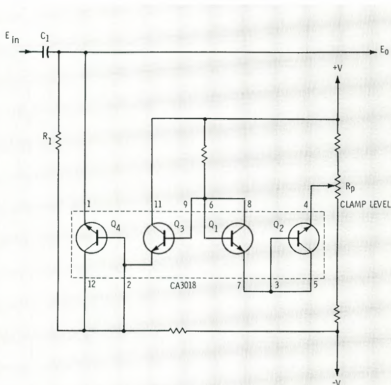
Fig. 2c Negative clamp with programmable reference level.
