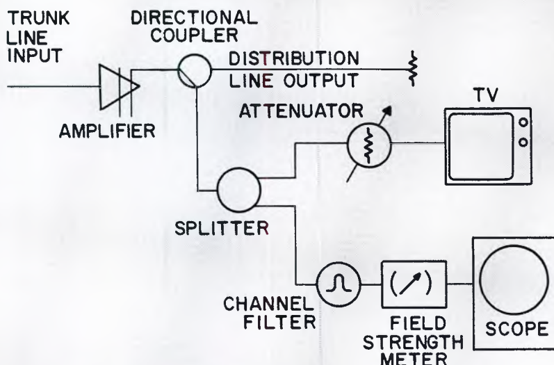
Fig. 1 Cross-modulation measurement of a CATV system.
