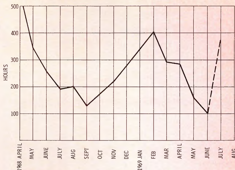
Fig. 1 Time and study of head life shows great difference between winter and summer months. Note that late 1969 months show results of tip adjustments.
