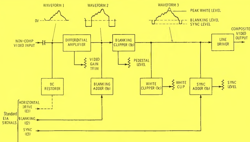
Fig. 6a Block diagram of video processor. (6b) Video processor system.
